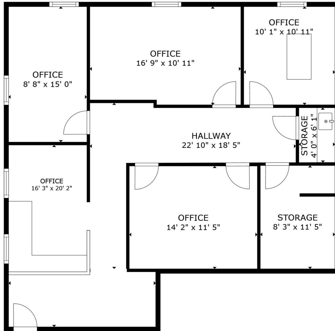
FLOOR PLAN
