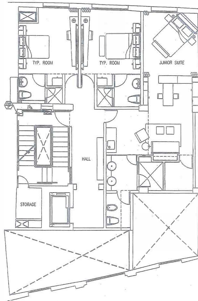
FIFTH LEVEL - FIRE PROTECTION LAYOUT SCALE: 1/4" = 1'-0"
