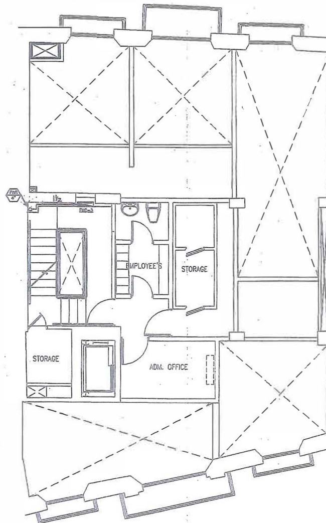
THIRD LEVEL - FIRE PROTECTION LAYOUT SCALE: 1/4" = 1'-0"
