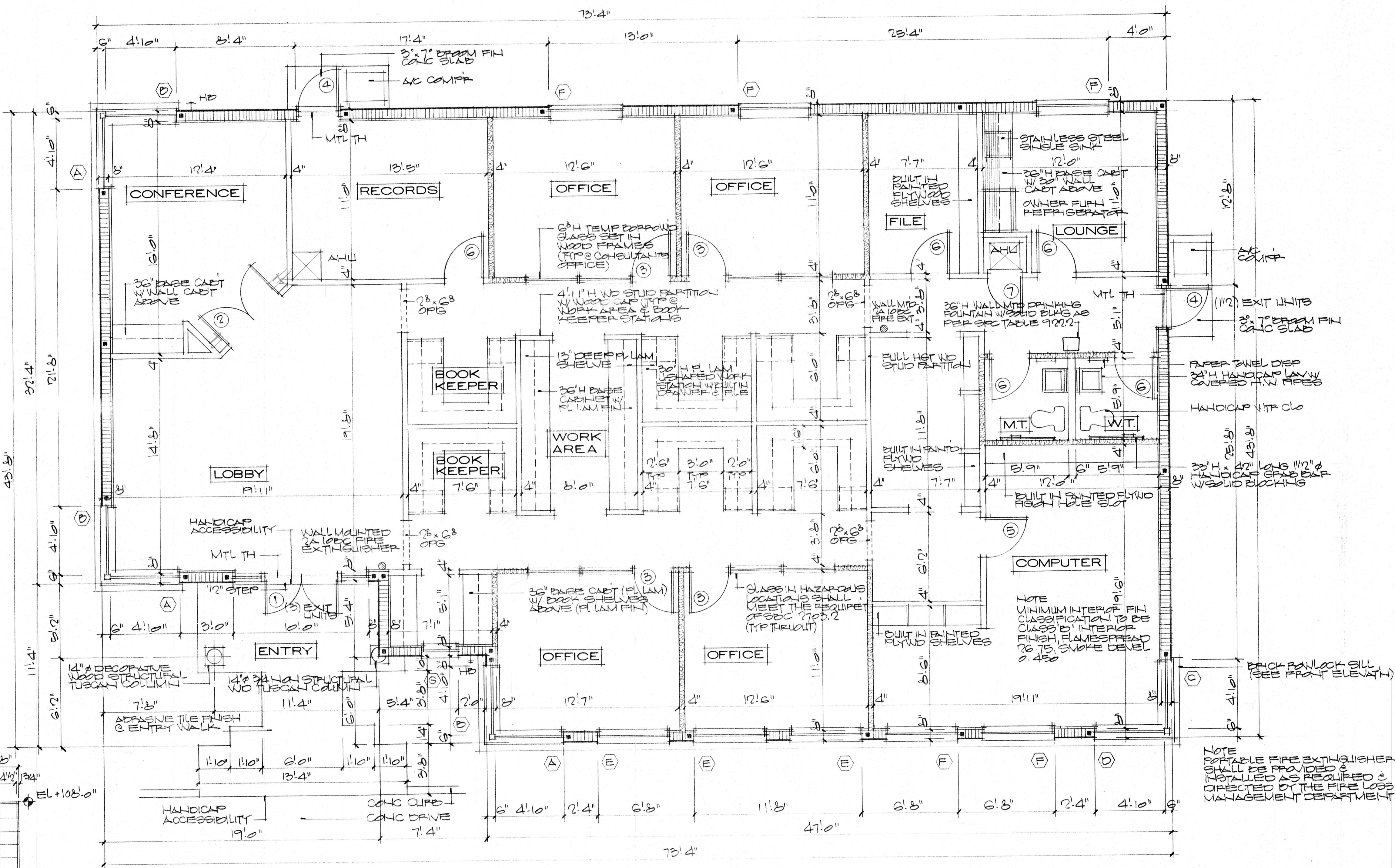
FLOOR PLAN
