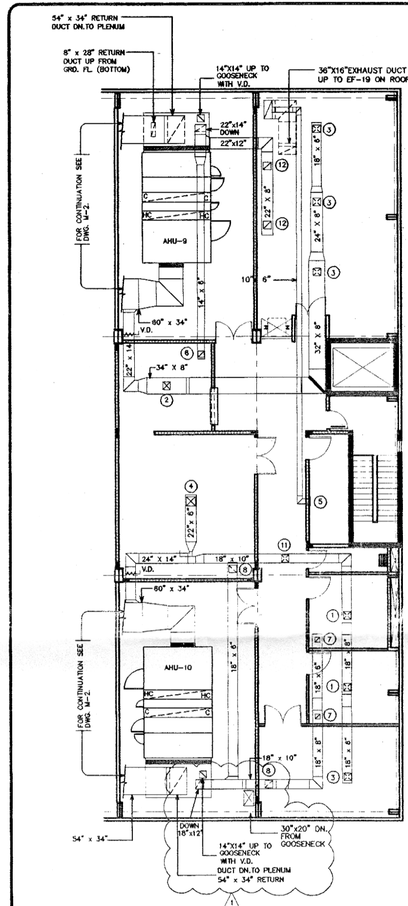
MEZZANINE ABOVE 2ND. FLOOR PLAN SCALE: 1/8" = 1' - 0"
