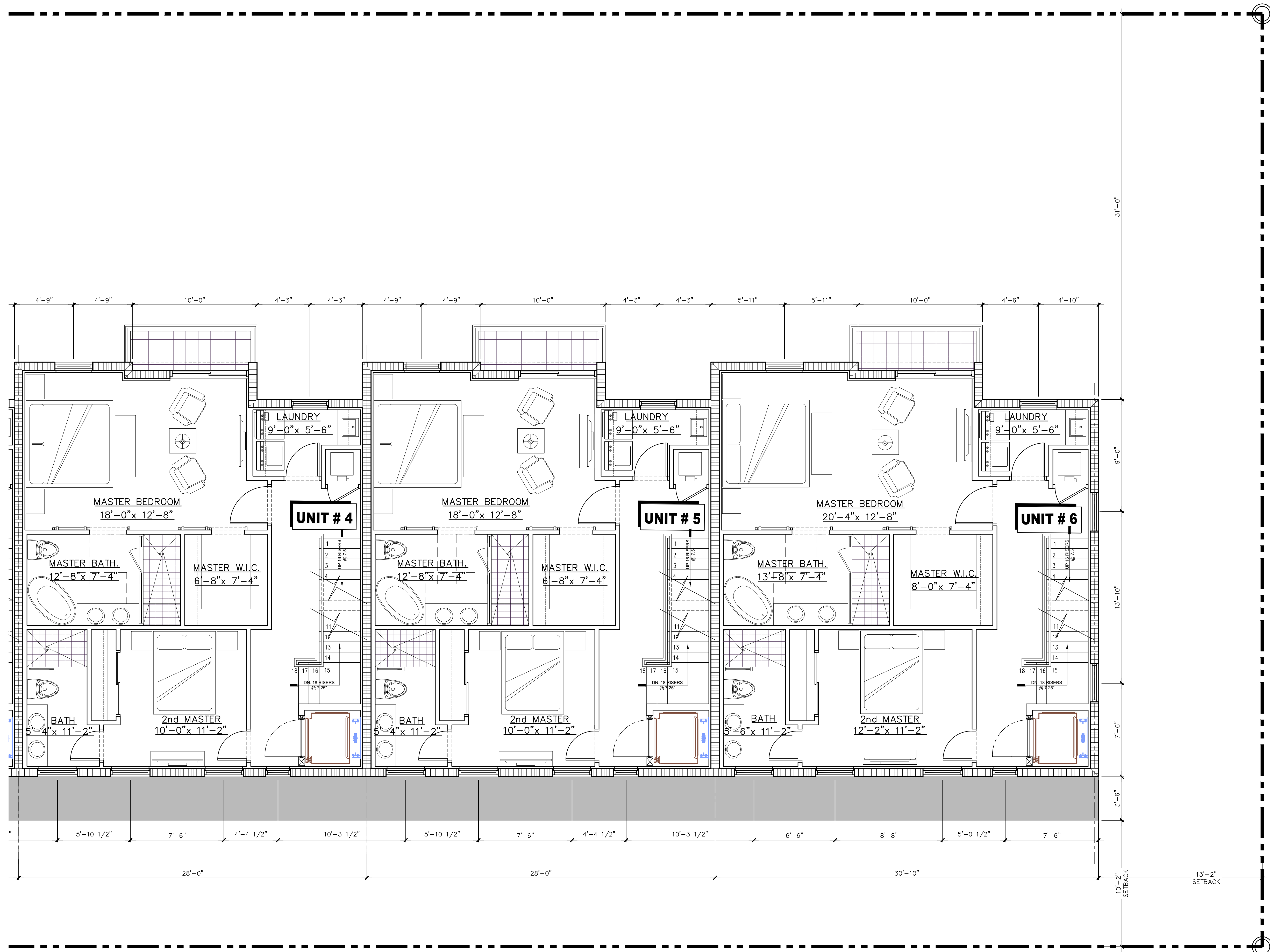
1 ENLARGED THIRD FLOOR UNITS #4,5,6 NORTH SCALE: 1"=1/4"
