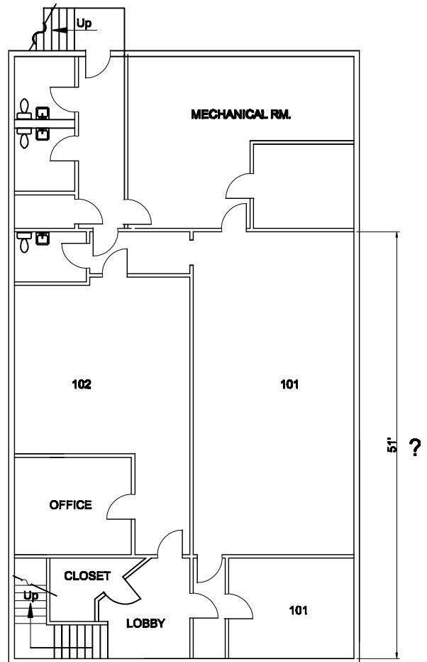
Floor Plan - Lower Level
