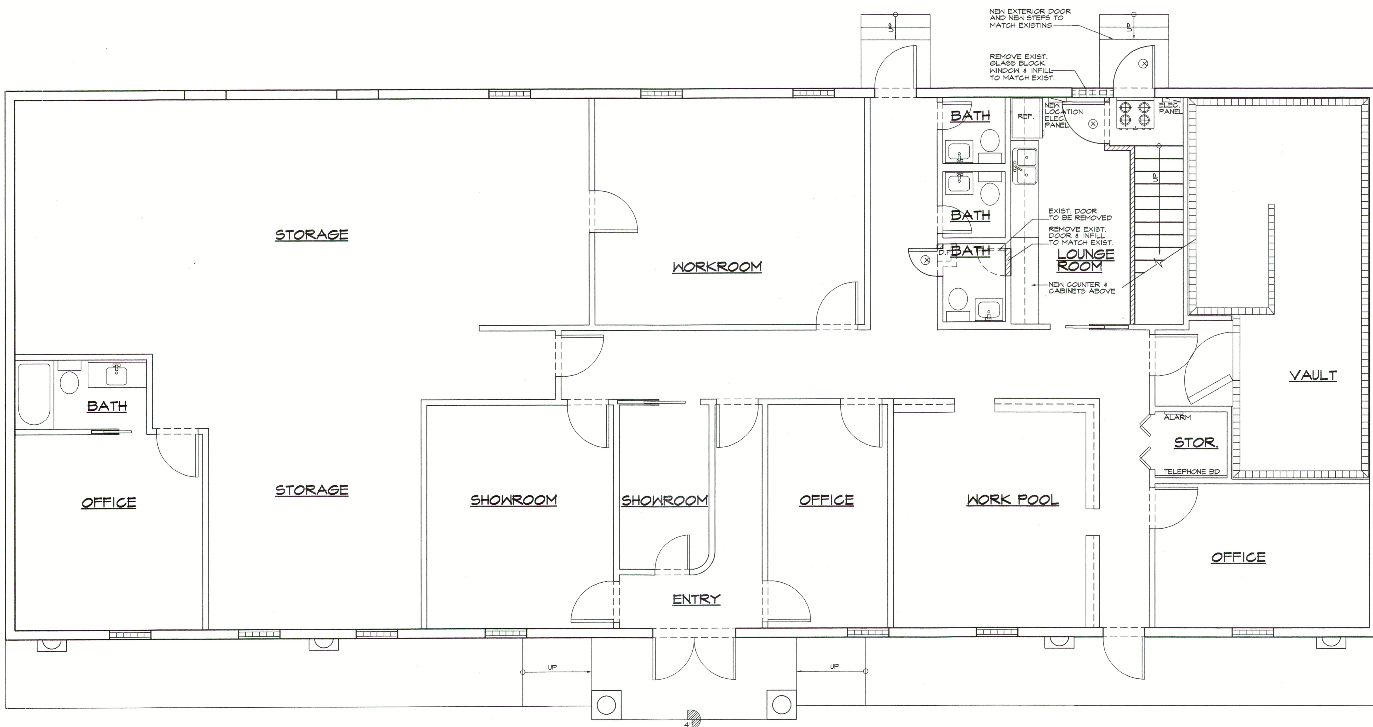
PROPOSED FIRST FLOOR PLAN SCALE: 1/4" = 1'-0"
