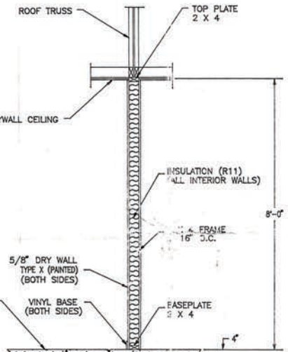
DETAIL 1 HR UL FIRE RATED WALL (DESIGN NO.: U305) MEDICAL SUPPLIES/STORAGE ROOMS
