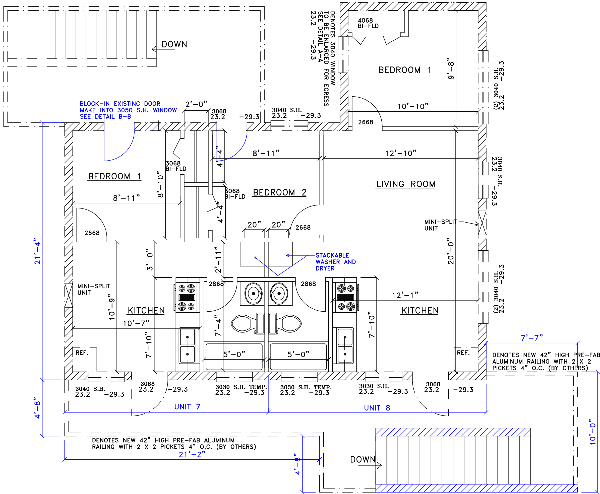
THIRD FLOOR PLAN UNIT 7,8 1/4"=1'-0"
