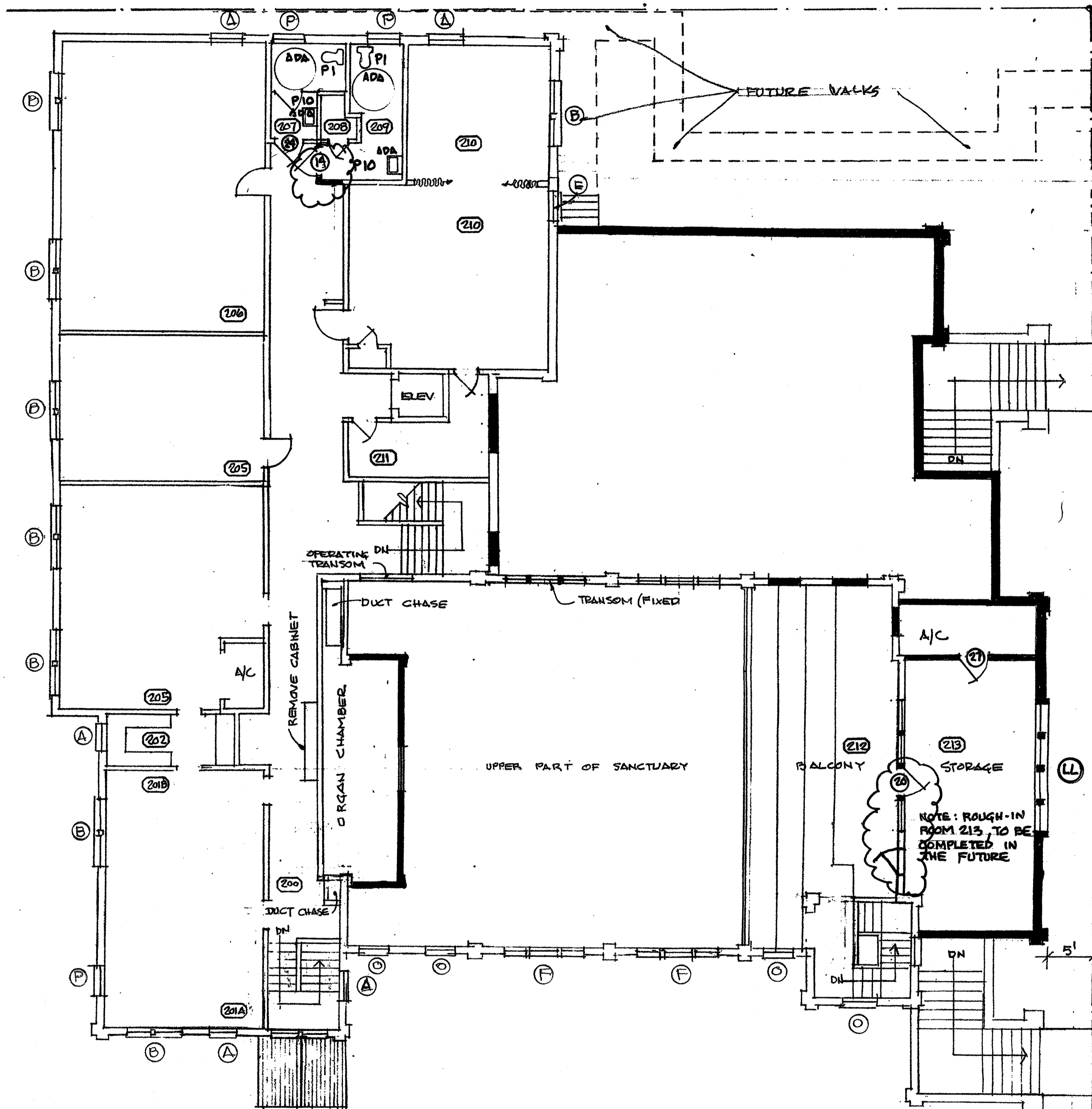
FLOOR PLAN - SECOND FLOOR - 1/8" = 1'-0" SHOWING POST-BID REVISIONS
