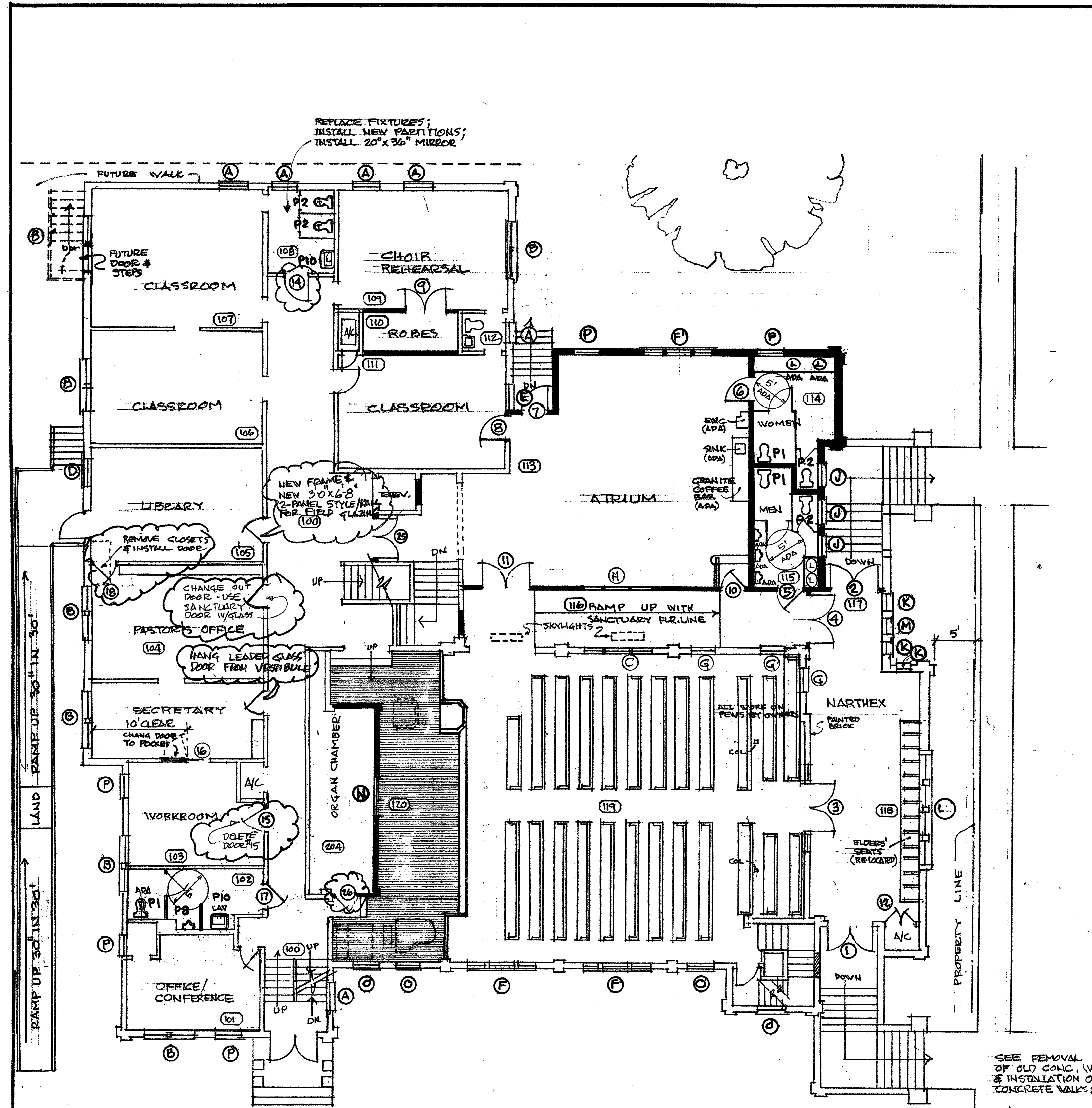
FLOOR PLAN • FIRST FLOOR • 1/8" = 1'-0" SHOWING POST-BID REVISIONS
