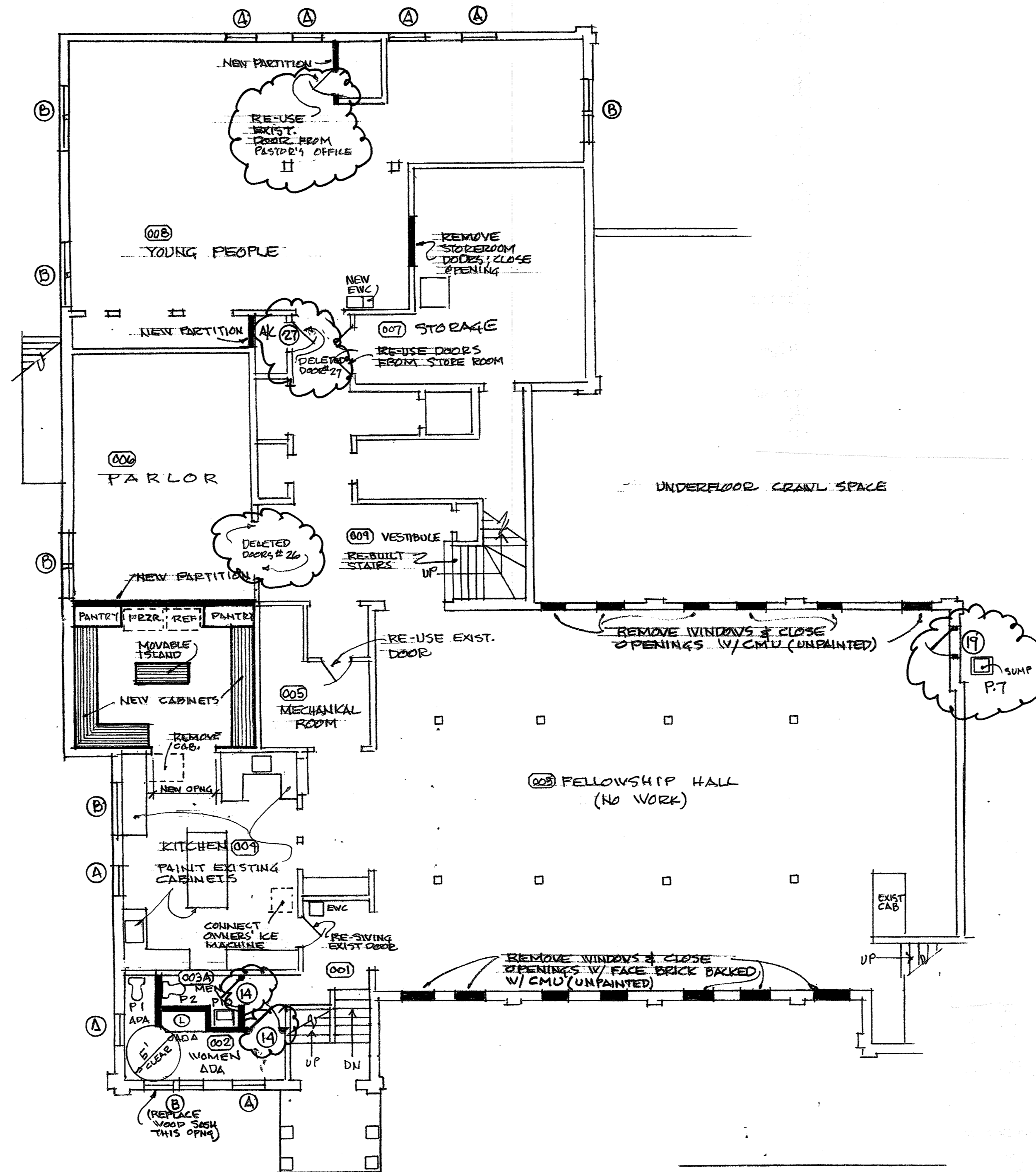
FLOOR PLAN • BASEMENT • 1/8" = 1'-0"
