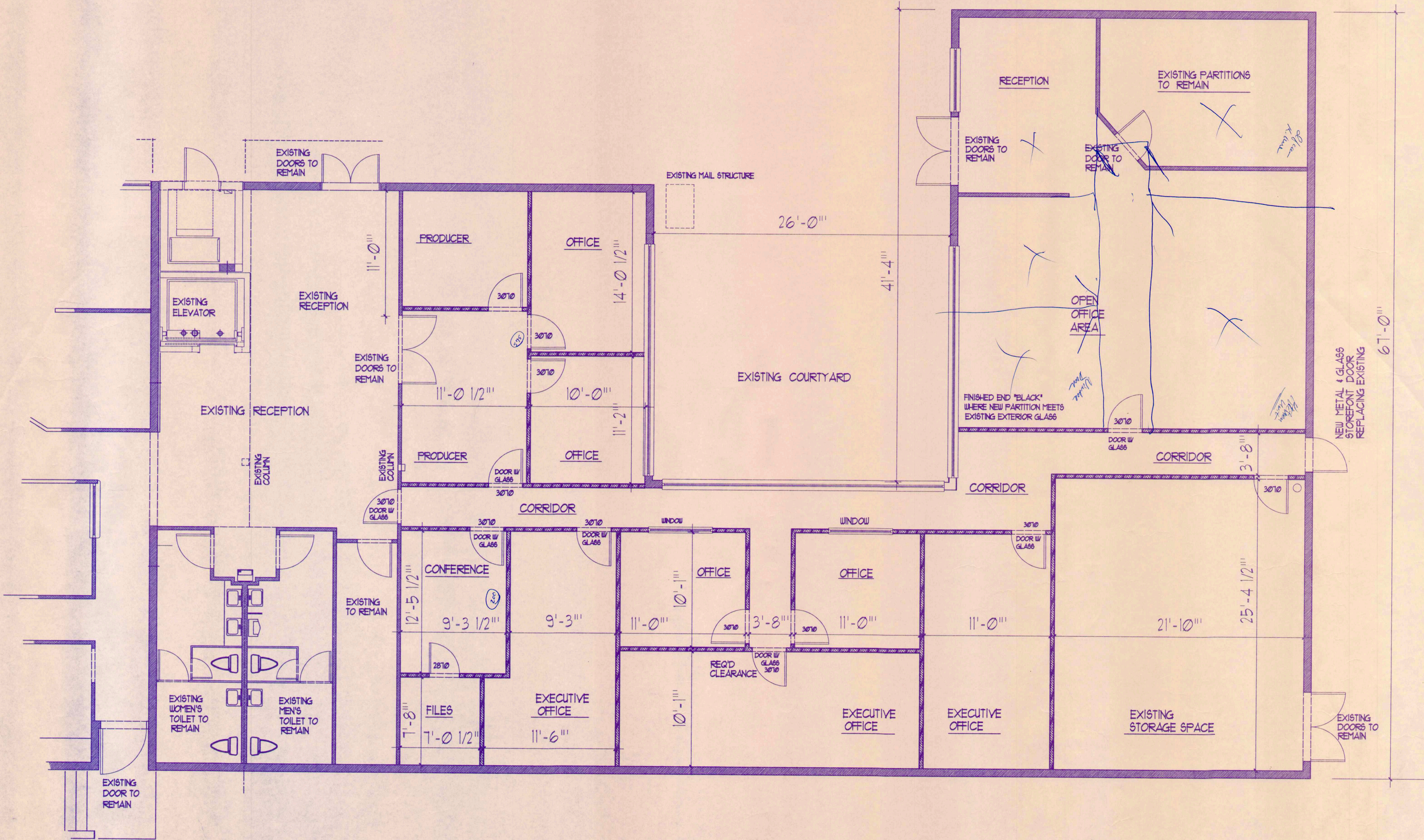
REMODELED 1st LEVEL FLOOR PLAN 3,926 SQ FT 1/4" = 1'-0"
