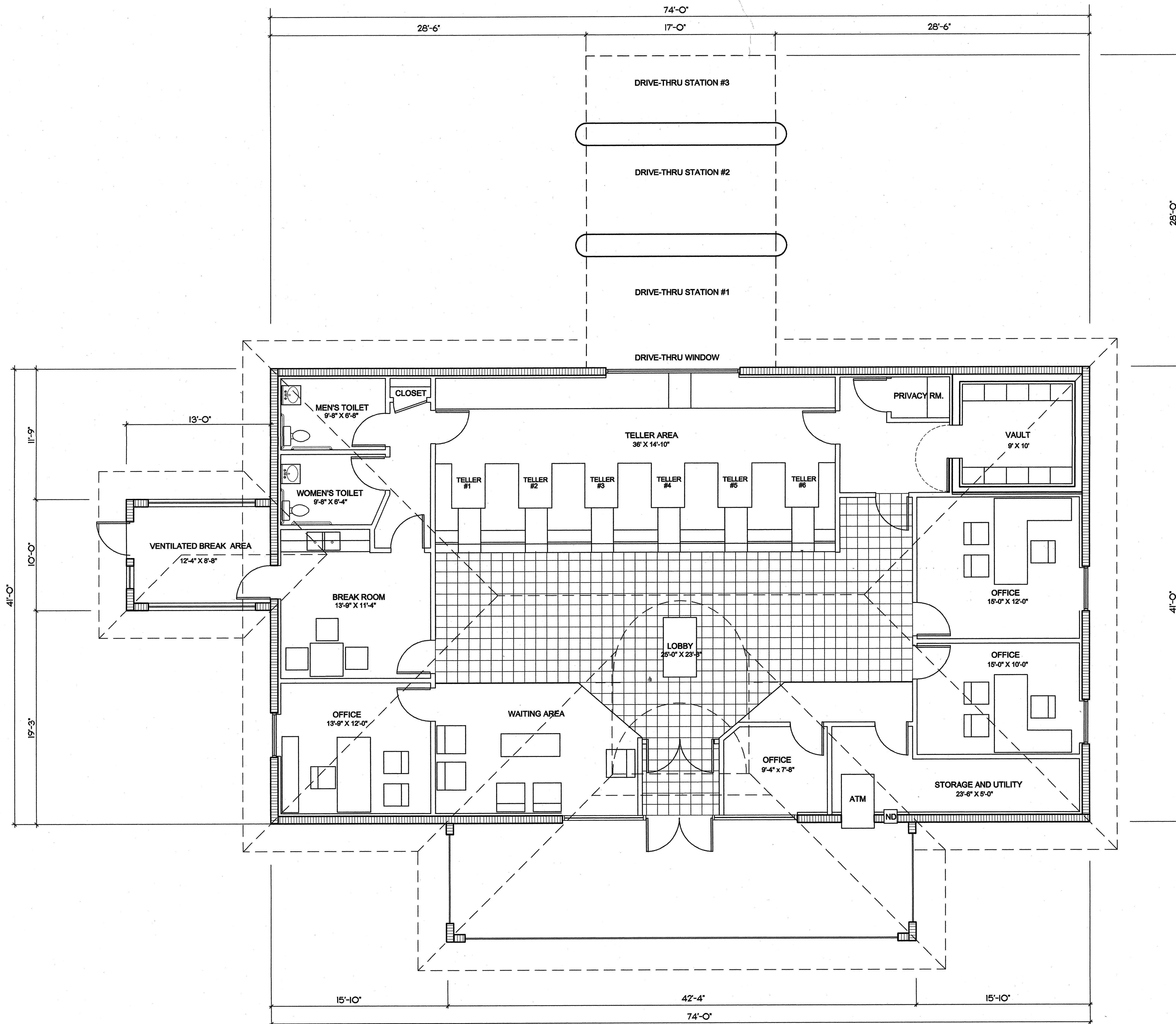
1 PRELIMINARY FLOOR PLAN - OPTION #2 STANDARD TELLER STATIONS 1/4" = 1'-0"
