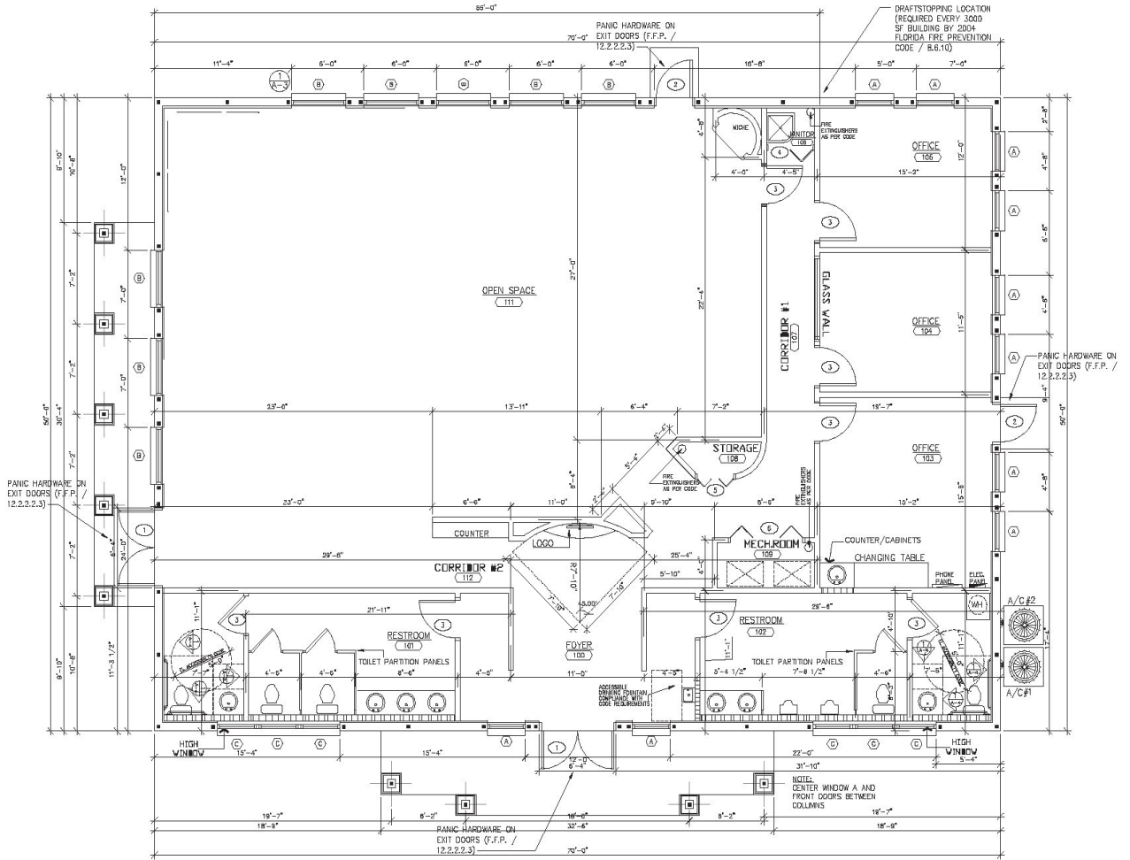
Floor Plan
