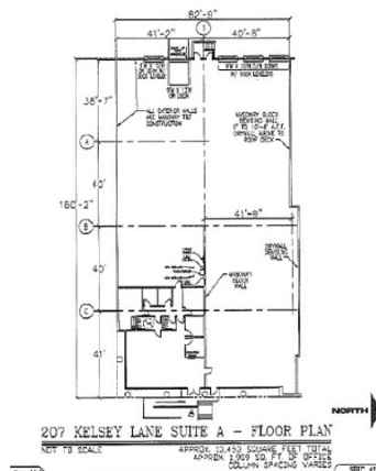
Suite A Floor Plan
