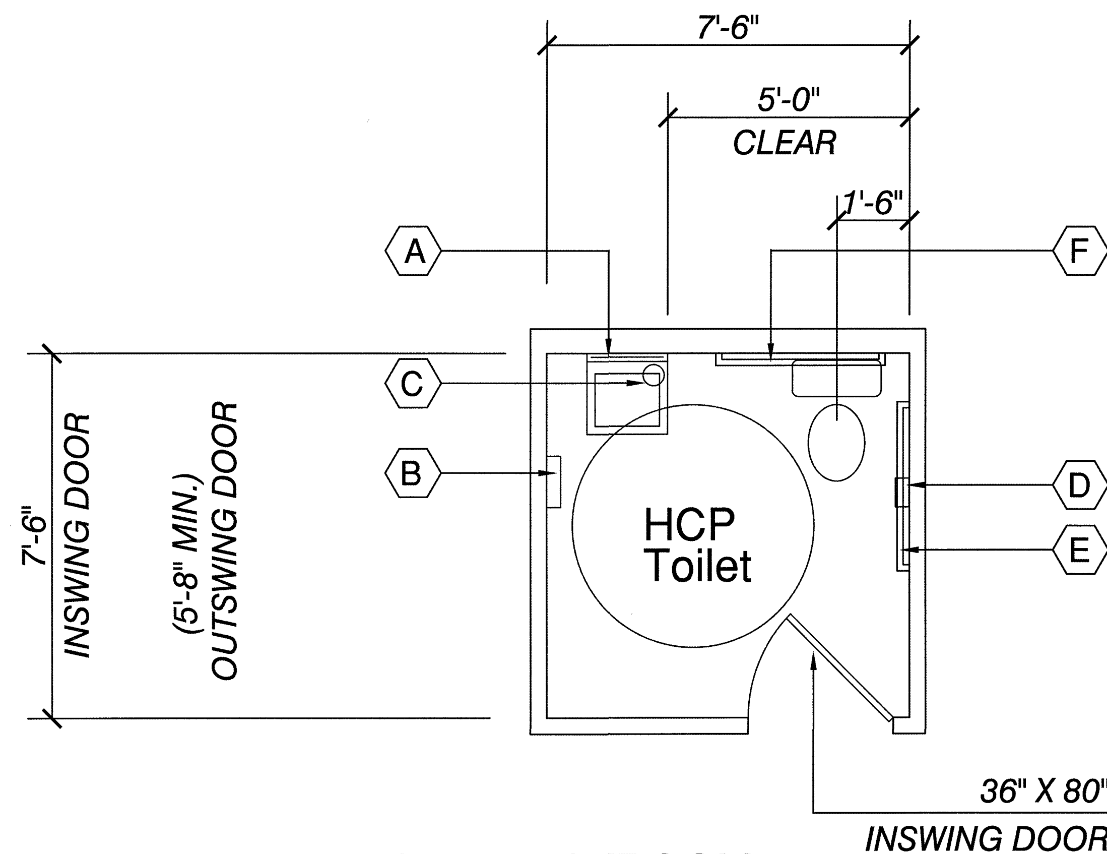
TYPICAL RESTROOM ADA SPECS
