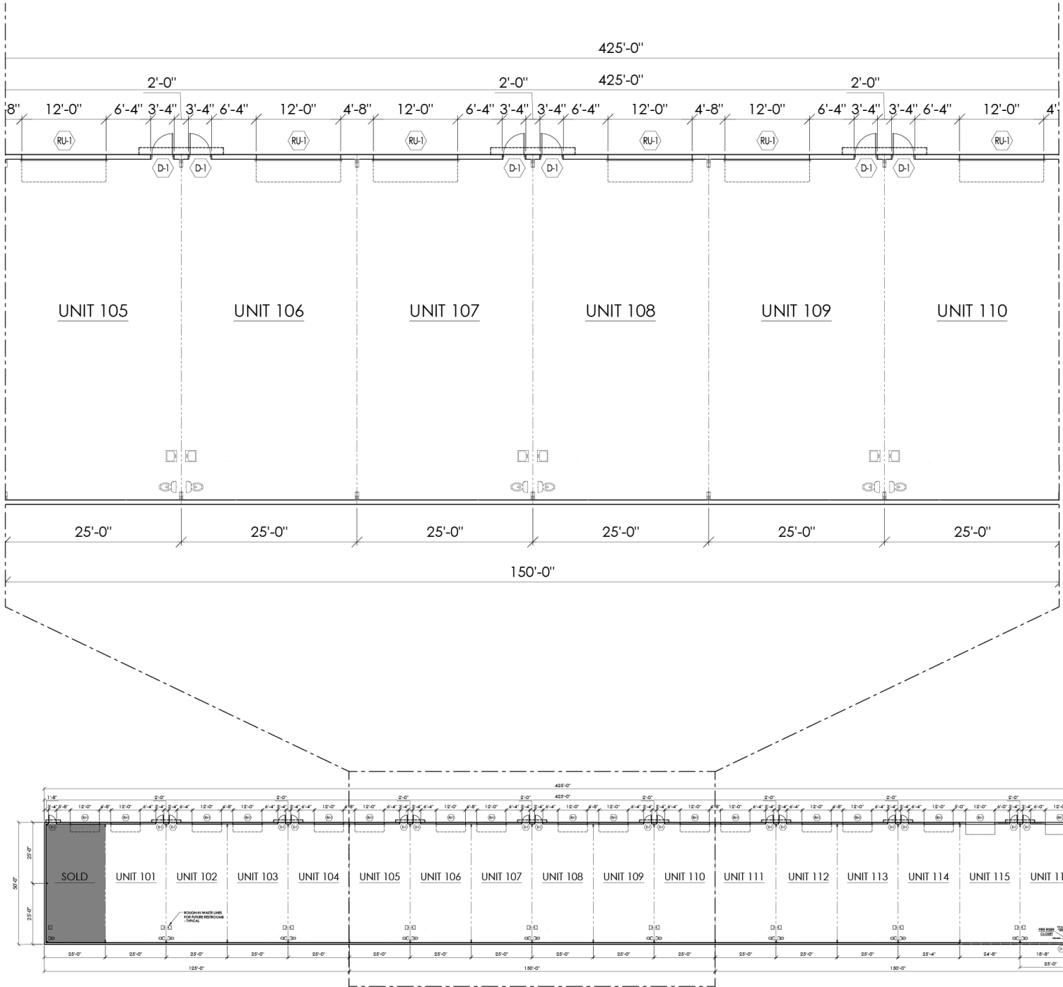
OVERALL FLOOR PLAN SCALE: 1/16" = 1'-0"
