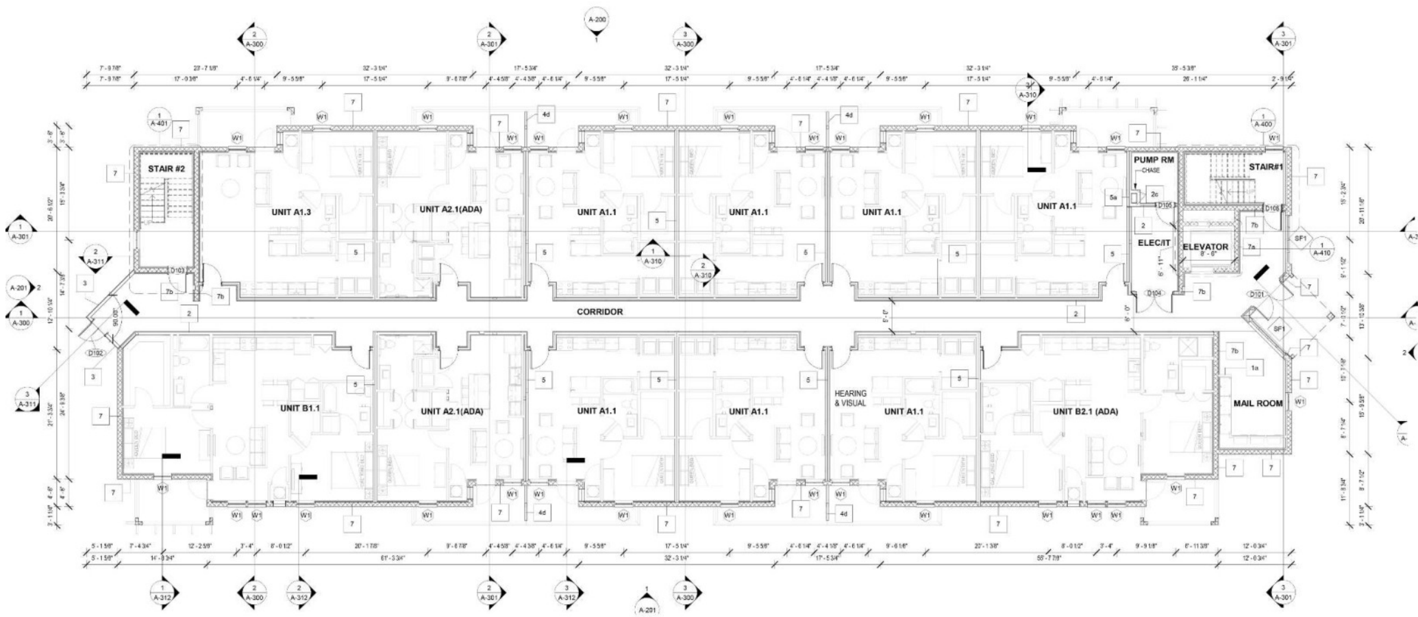
1 FIRST FLOOR OVERALL PLAN* 1/8" = 1'-0"
