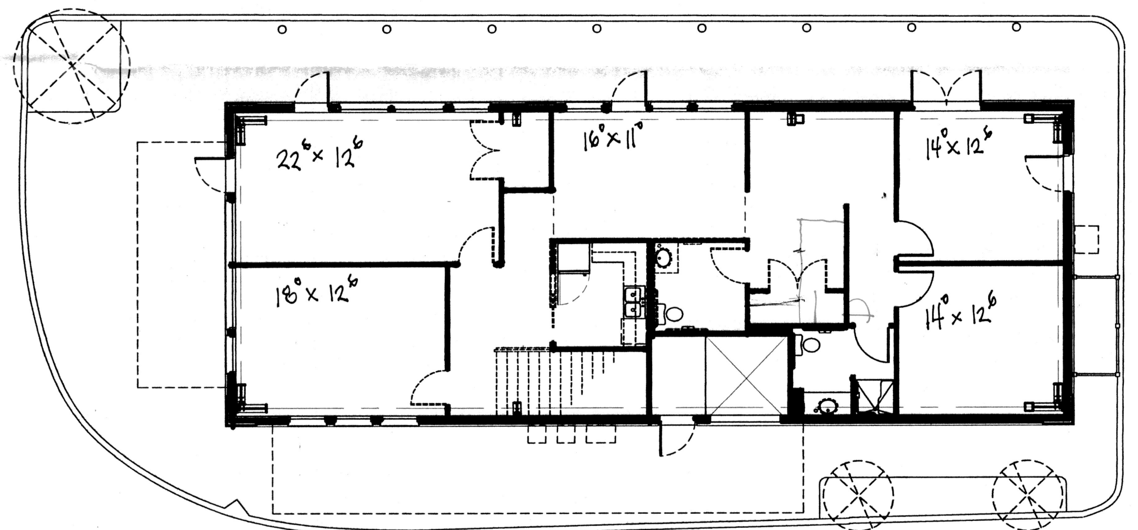
First Floor
