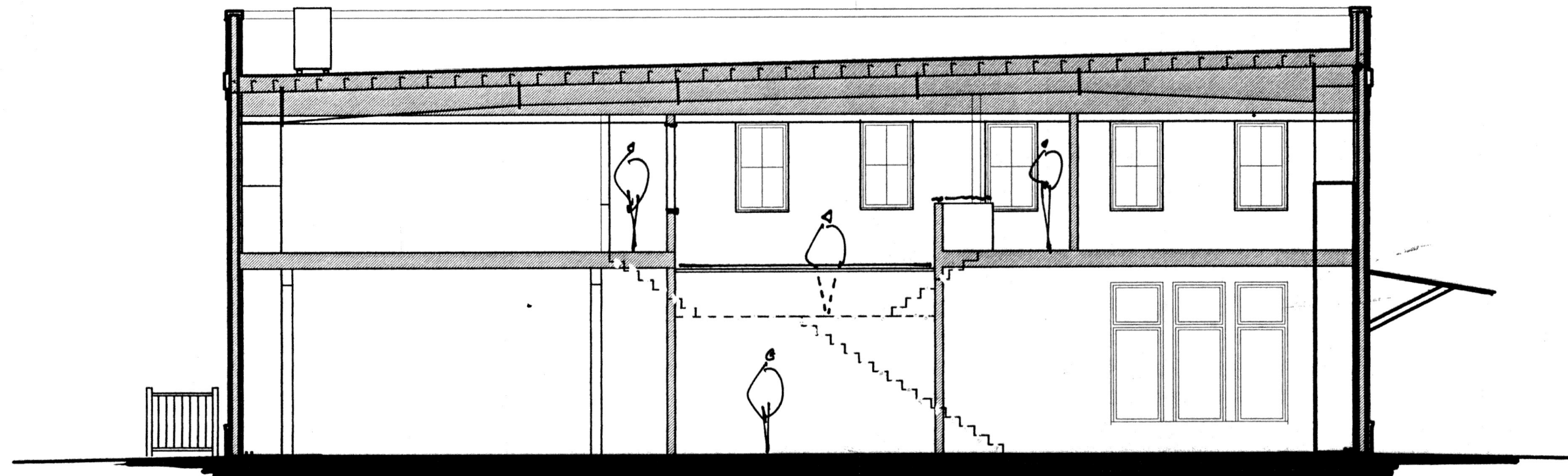
Building Section
