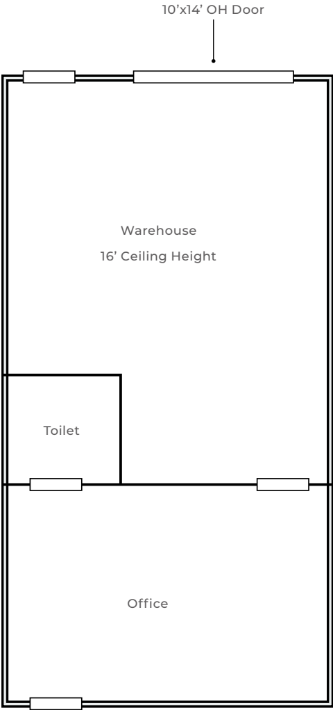
FLOORPLAN - UNIT 6B
