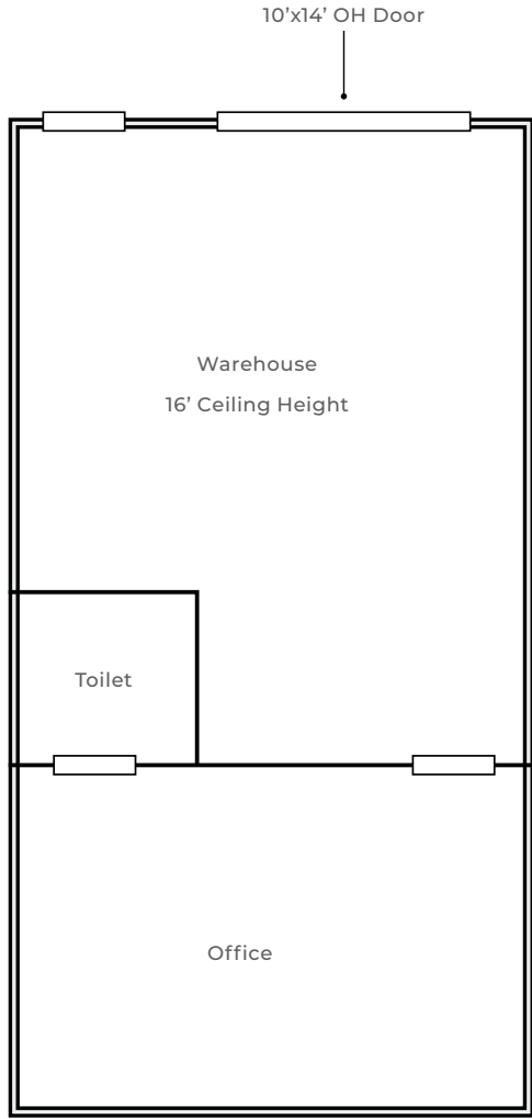
FLOORPLAN - UNIT 8A
