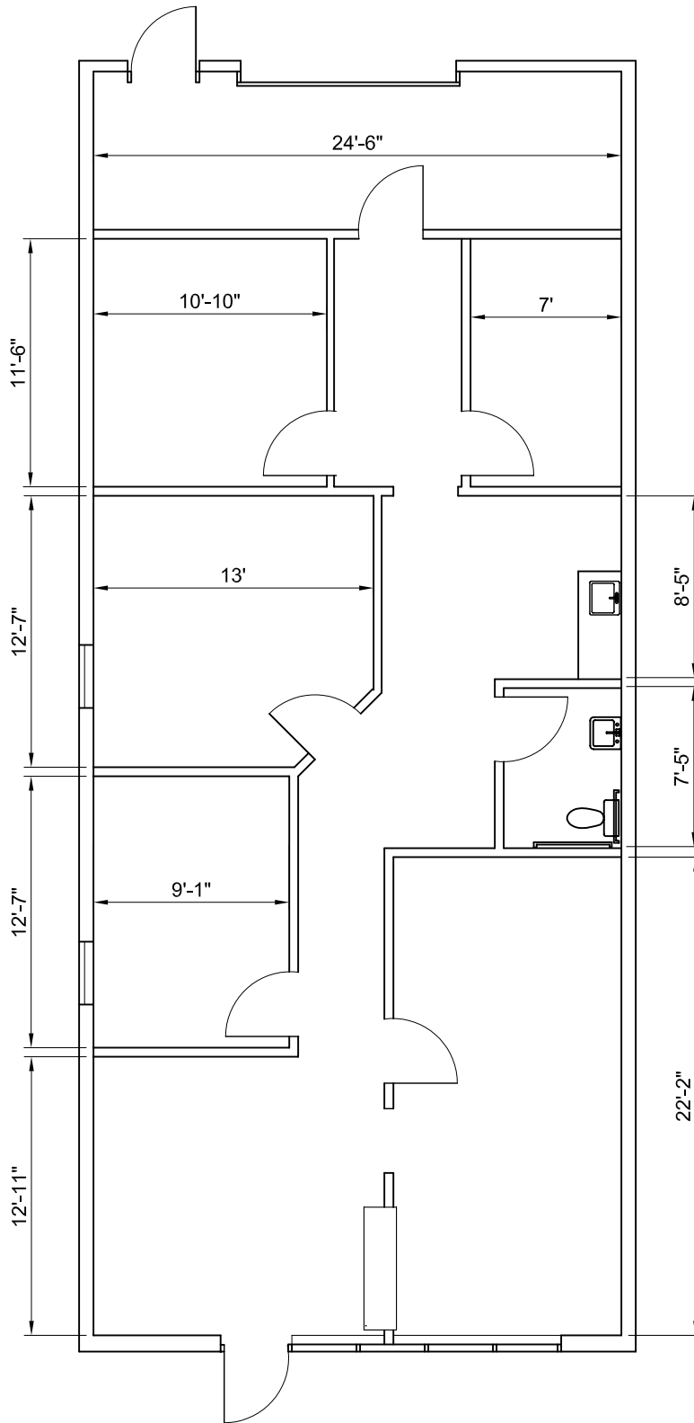
Floor Plan Suite 700 1/8" = 1'-0" 1,492 SF
