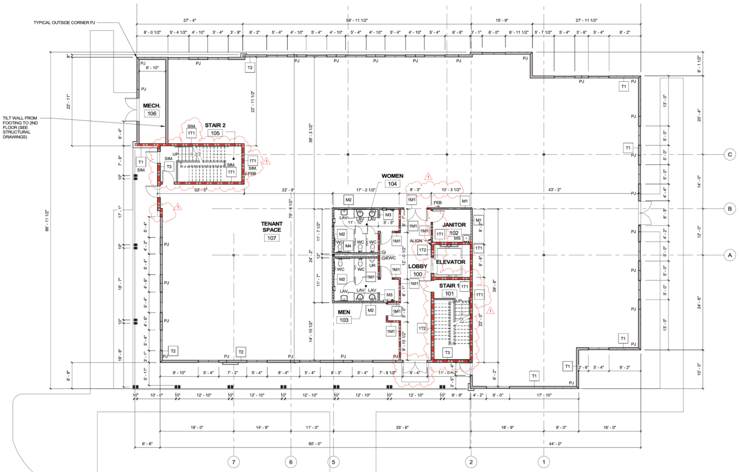
Building Shell (First Floor)
