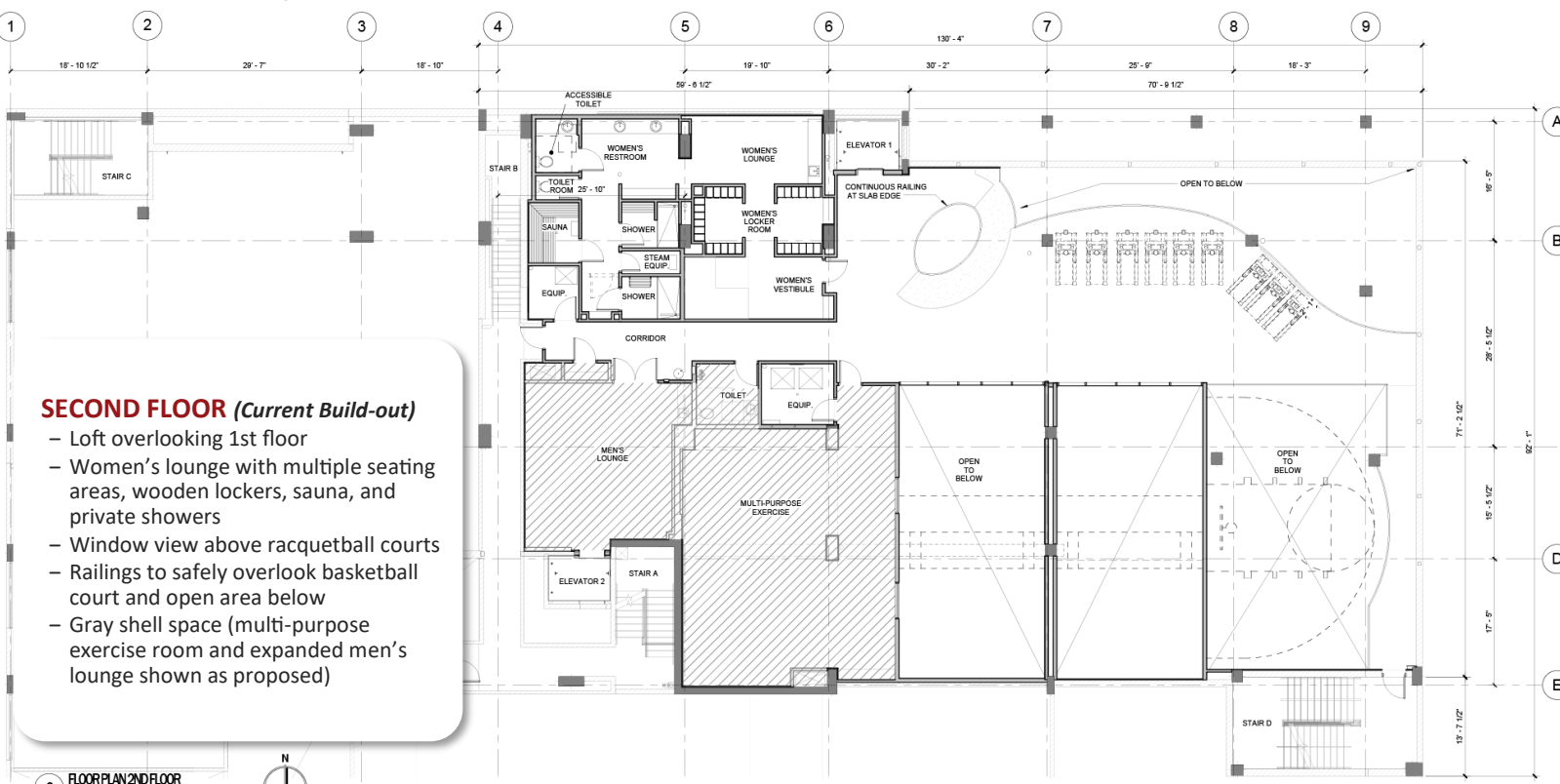
2 FLOOR PLAN 2ND FLOOR 1/8" = 1'-0"
