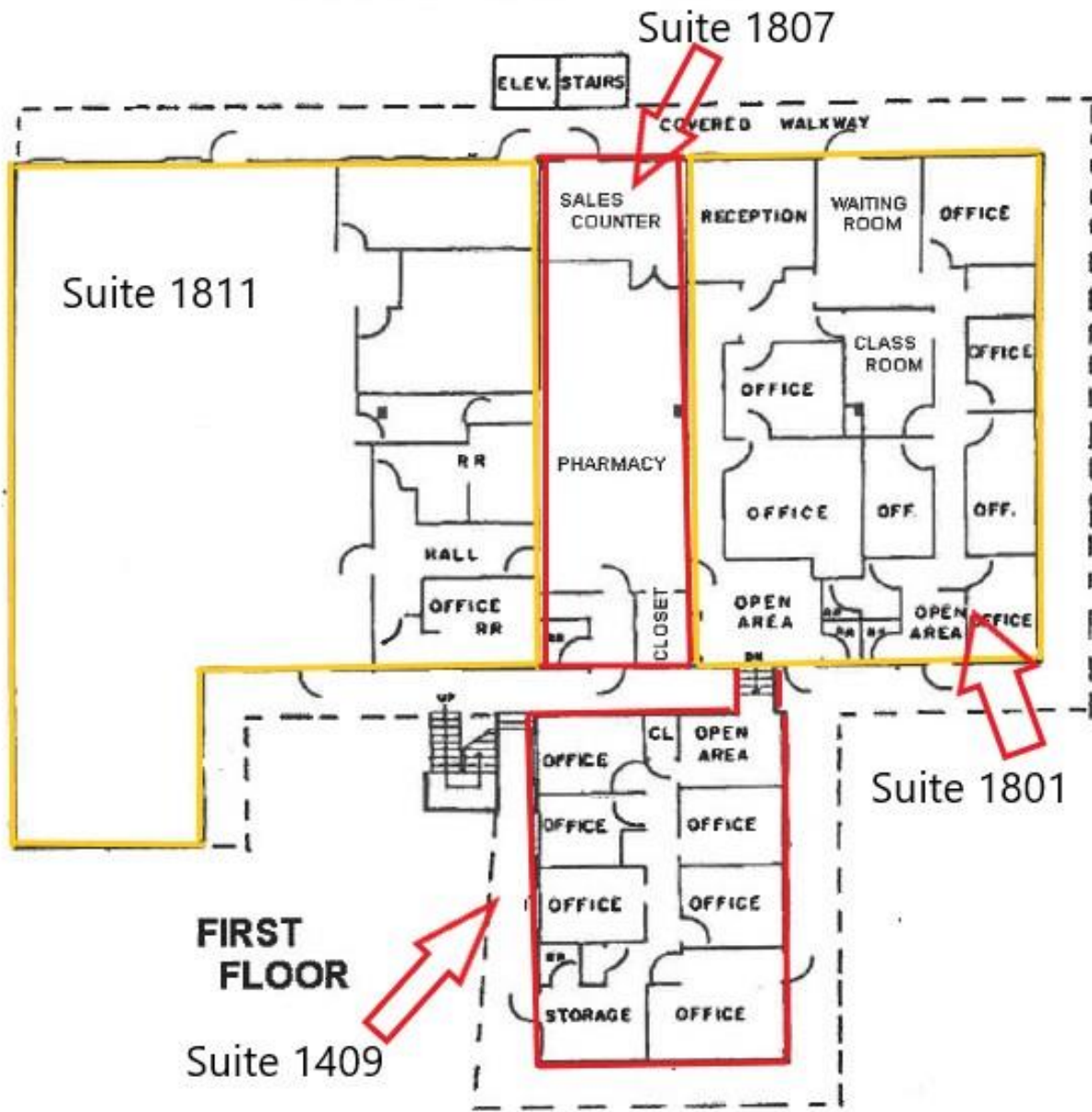
BUILDING FLOOR PLAN - 1 ST FLOOR
