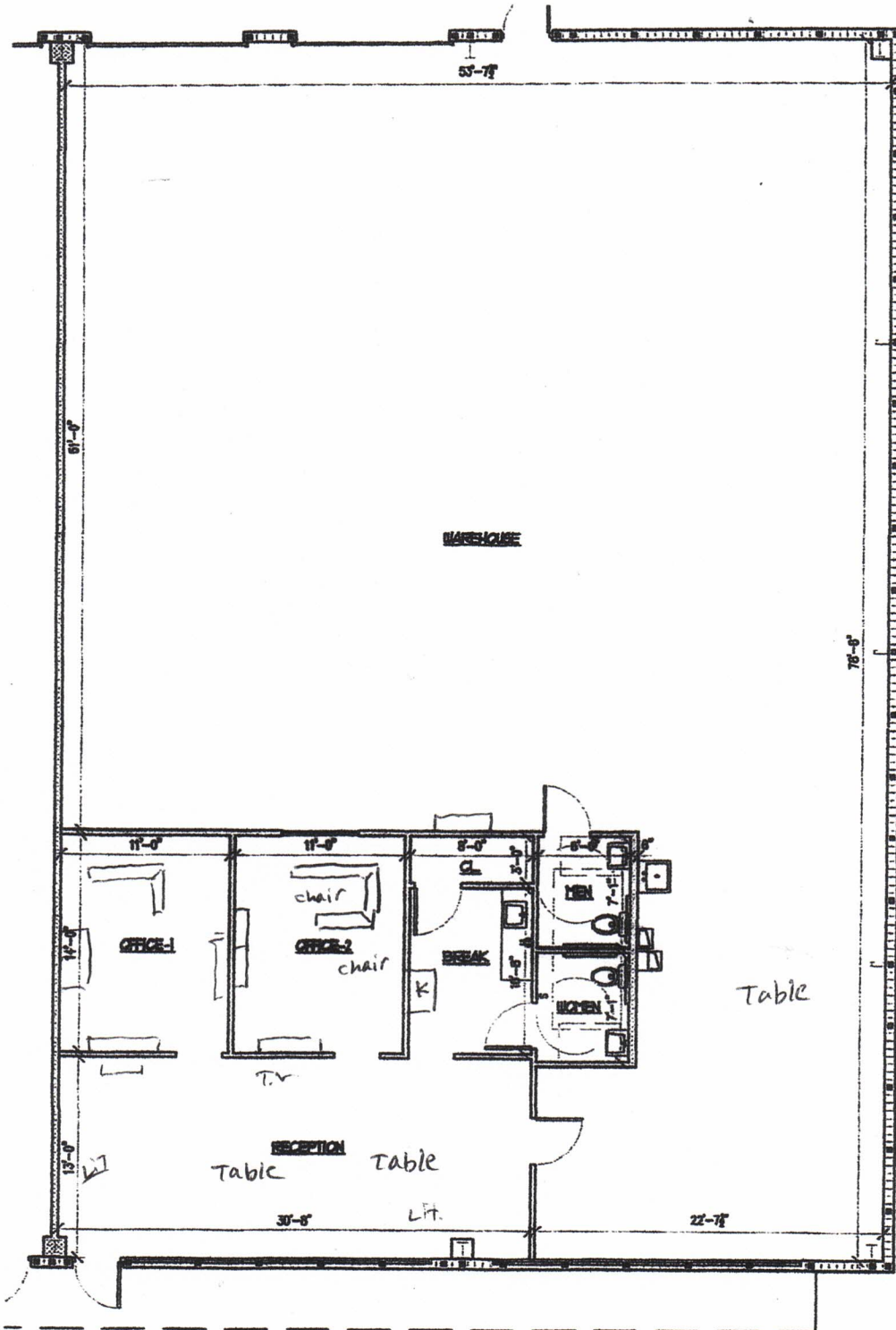
1 FLOOR PLAN (4,360 SF.) SCALE: 3/32" = 1'-0"
