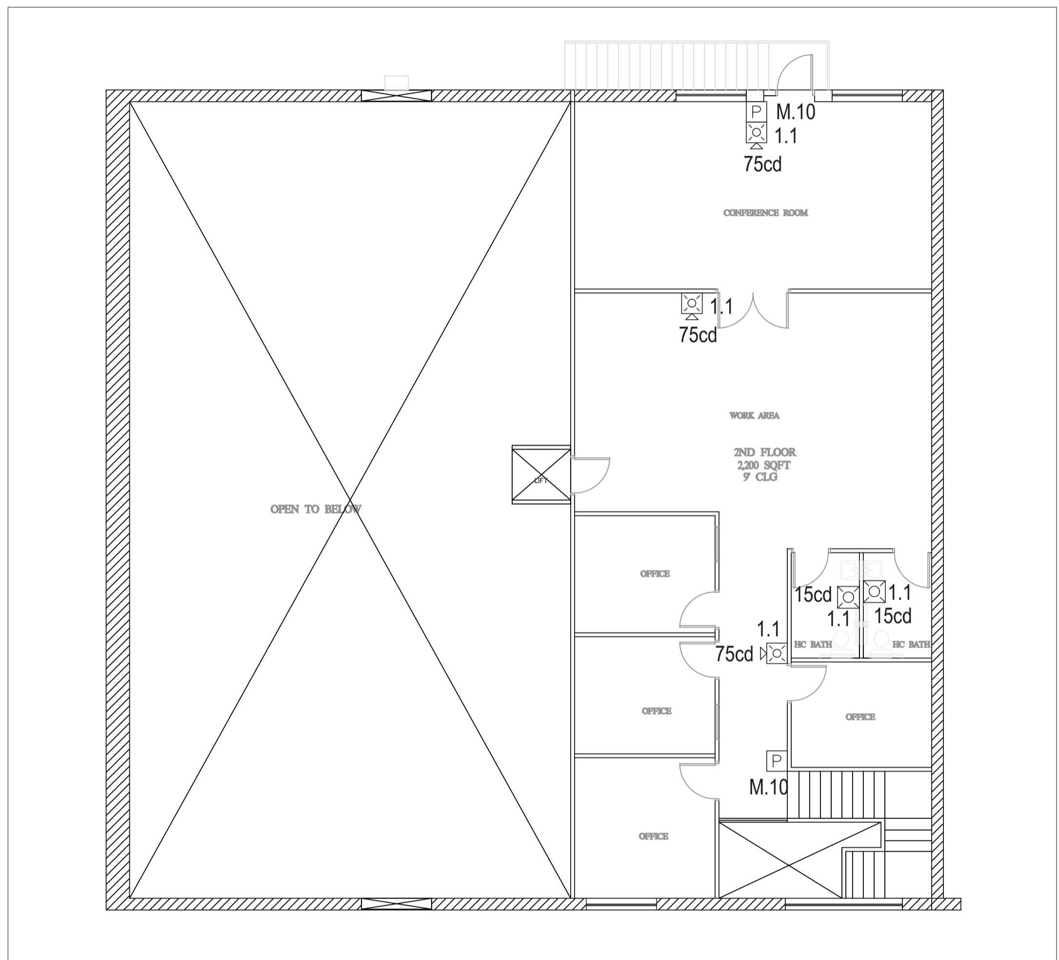
MEZZANINE FIRE ALARM FLOOR PLAN
