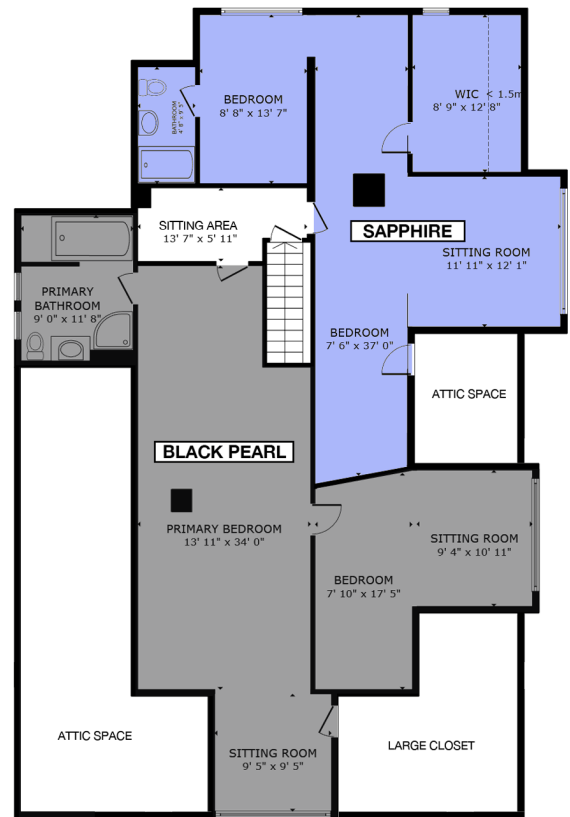
FLOOR 3
