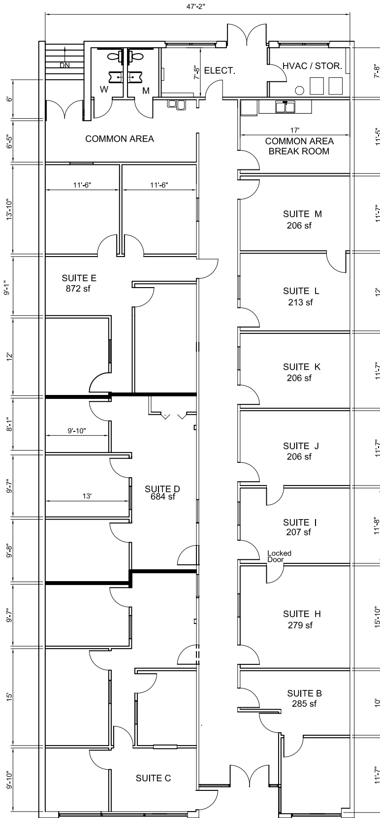
Floor Plan No Scale
