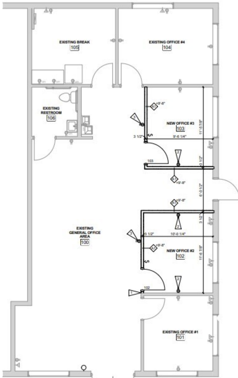
1 PLAN FIRST FLOOR / POWER 1/4" = 1'-0" 223 SF ALTERATION
